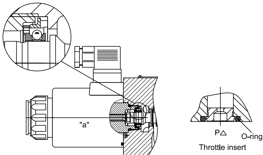
Type:WE10.L5X/OF ... (Impulse spool)
