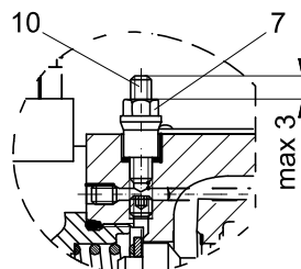
With throttle crew 'C'
