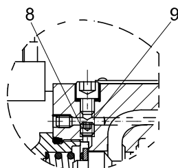
With orifice 'A0.'
