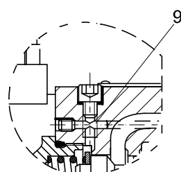
Without throttle screw/ without orifice
